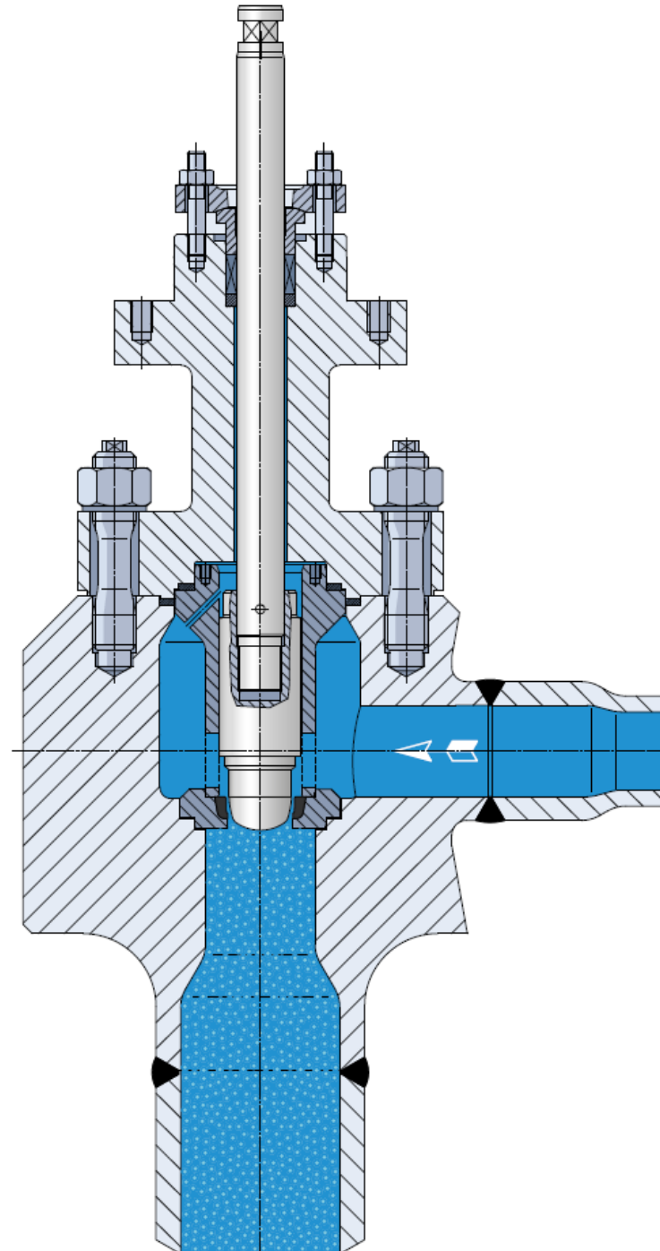
Typical drain valve, separated seat and control, clamped trim Forged body, increased diameter outlet
