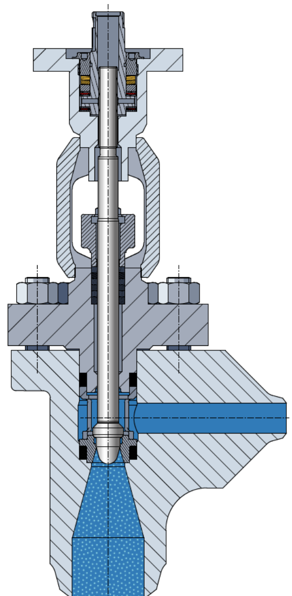
Typical drain on-off valve, separated seat and control, clamped trim Forged body, increased diameter outlet
