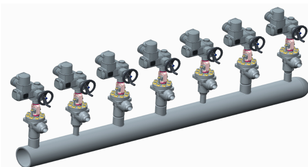
Typical drain on-off valve, separated seat and control, clamped trim Forged body, increased diameter outlet
